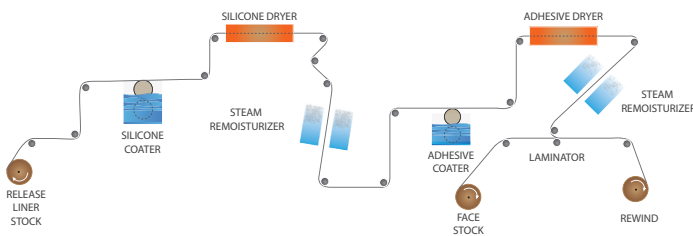
Figure 1: Typical Label Manufacturing Process
